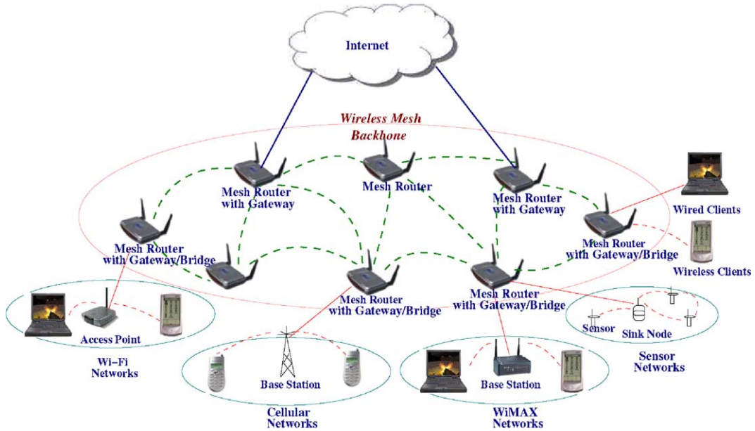
Fig. 3. Infrastructure/backbone WMNs.
